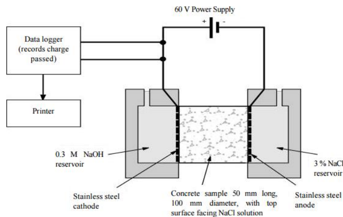
Figure 5. Rapid Chloride Permeability Test Setup [15, 16]
